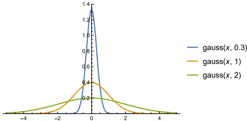
Figure 3.2 The Gaussian function at scales \sigma = .3, \sigma = 1 and \sigma = 2 . The kernel is normalized, so the total area under the curve is always unity.
