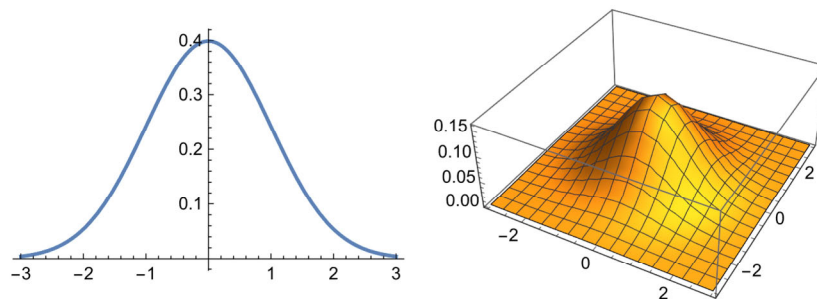
Figure 3.7 A product of Gaussian functions gives a higher dimensional Gaussian function. This is a consequence of the separability.
