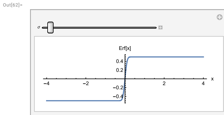
Figure 3.5 For decreasing \sigma the Error function begins to look like a step function. The Error function is the Gaussian blurred step-edge.
