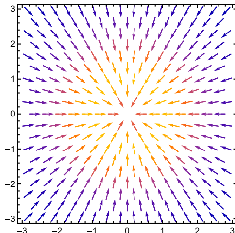
Figure 3.15 The slope of an isotropic Gaussian function is indicated by arrows here. There are circularly symmetric, i.e. in all directions the same, from which the name isotropic
