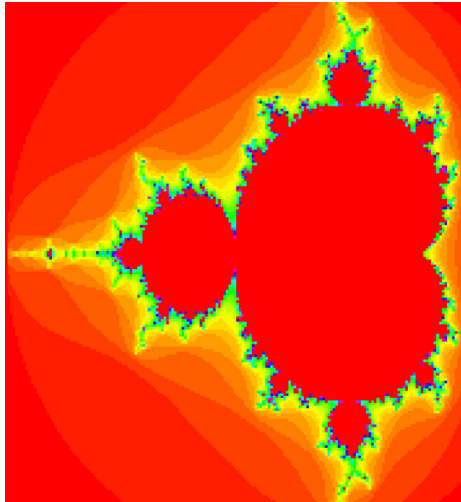
Figure 3.3 The Mandelbrot fractal is a famous example of a self-similar function. See also mathworld.wolfram.com/MandelbrotSet.html and MandelbrotSetPlot in the Wolfram Documentation.
