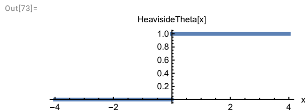
Figure 3.6 The Heaviside function is the generalized unit stepfunction. It is the limiting case of the Error function for \lim \sigma \rightarrow 0 .
