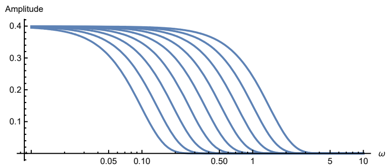
Figure 3.11 Fourier spectra of the Gaussian kernel for an exponential range of scales \sigma = 1 (most right graph) to \sigma = 14.39 (most left graph). The frequency \omega is on a logarithmic scale. The Gaussian kernels are seen to act as low-pass filters.
