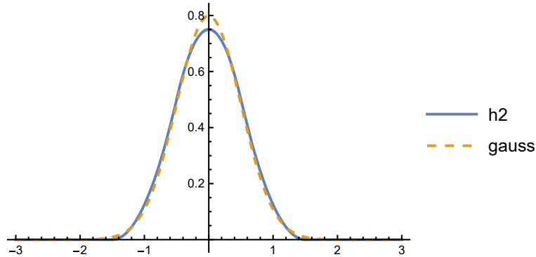
Figure 3.14 Two times a convolution of a blockfunction with the same blockfunction gives a function that rapidly begins to look like a Gaussian function. A Gaussian kernel with \sigma = 0.5 is drawn (dotted) for comparison.
