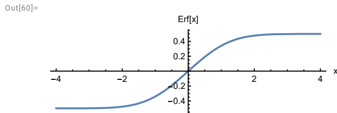
Figure 3.4 The error function Erf[x] is the cumulative Gaussian function.
