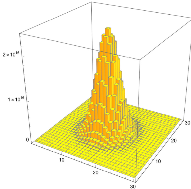
Figure 3.9 Binomial coefficients approximate a Gaussian distribution for increasing order. Here in 2 dimensions we see separability again.
