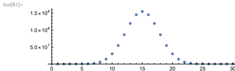
Figure 3.8 Binomial coefficients approximate a Gaussian distribution for increasing order.
