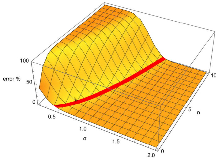
Figure 7.4 Relation between scale \sigma , order of differentiation n , and accepted error (in %) for a convolution with a Gaussian derivative function, implemented through the Fourier domain.
