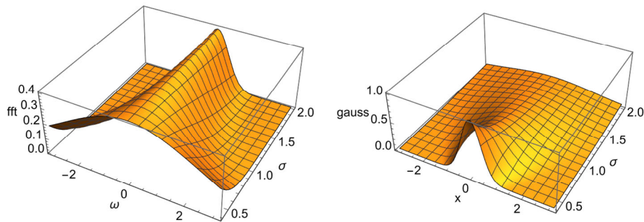
Figure 7.2 Left: The Fourier transform of the Gaussian kernel is defined for -\pi < \omega < \pi . The function repeats forever along the frequency axis over this domain. For decreasing scale \sigma in the spatial domain the Fourier transform get wider in the spatial frequency domain. At some value of \sigma a significant leakage (aliasing) occurs. Right: The spatial Gaussian kernel as a function of scale.
