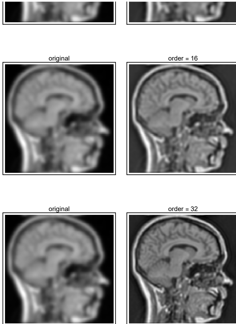
Figure 16.2 Deblurring of a blurred image ( 128^2 pixels, \sigma_{\text{blur}} = 2 pixels, left column) with different orders of approximation. The 32 nd order (bottom right) result comes close to the original (figure 16.1, left).
