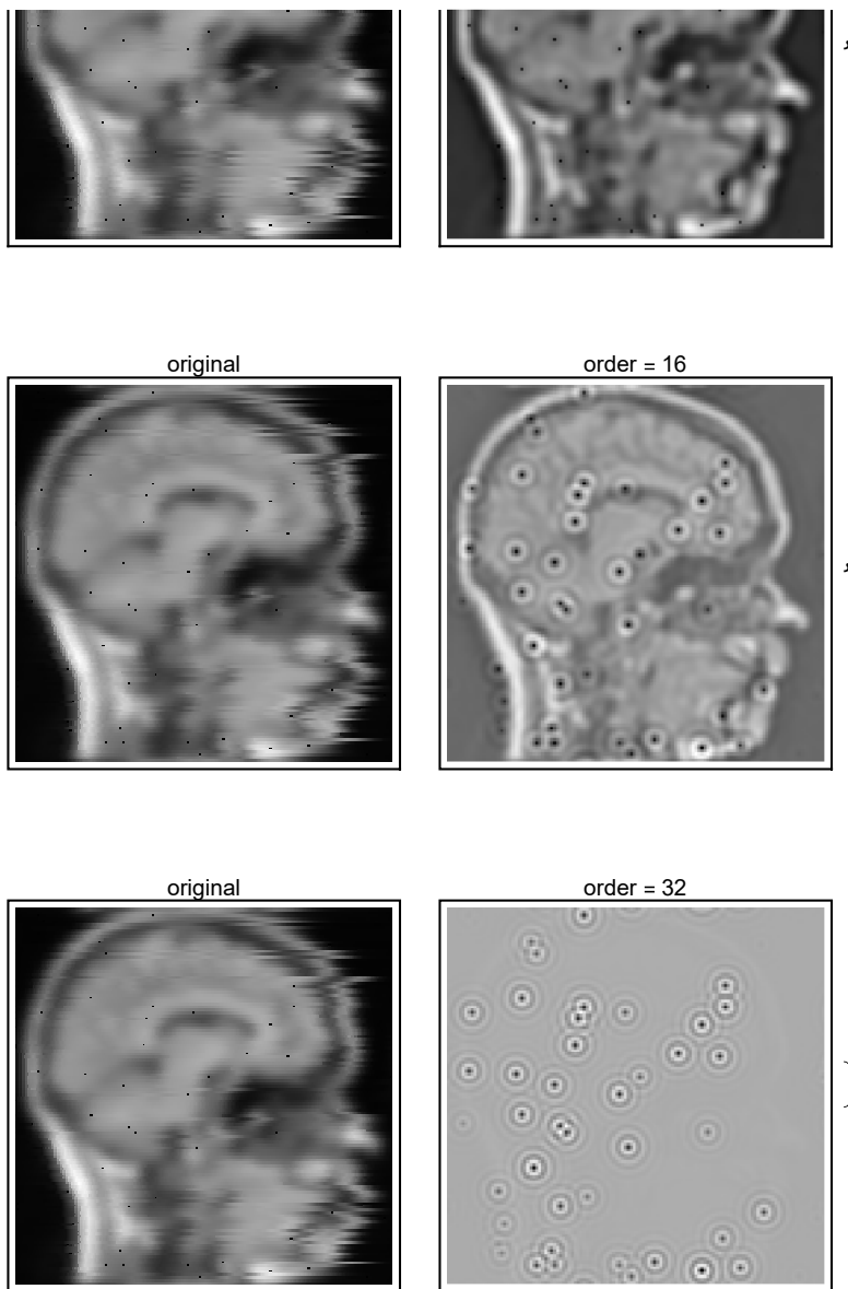
Figure 16.5 Deblurring results when the blurred image is disturbed by setting a random selection of 25 pixels to zero. The deblurring order is indicated with each result. Note that up to order 8 the 'blanked' points reconstruct well. At order 16 an overshoot occurs.
